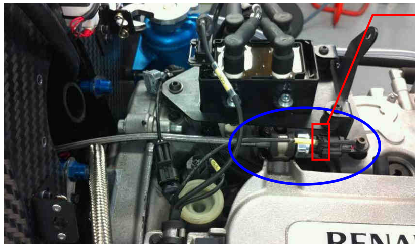
The Tie-wrap is strongly recommended for the reliability of the wires
