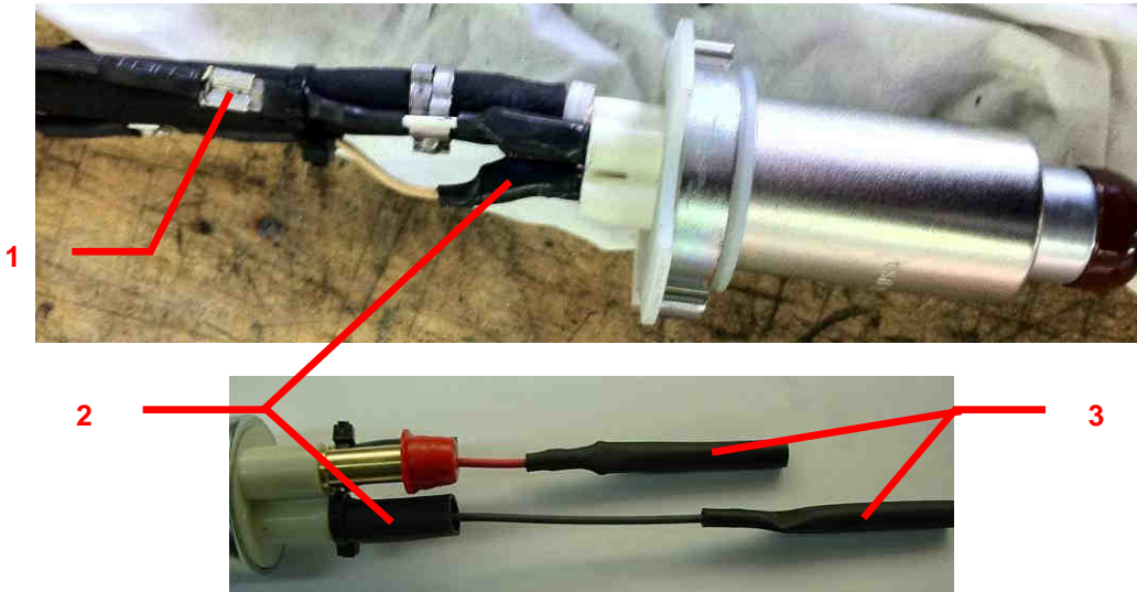
Fly wires welded and bonded on fuel pump terminals. Glue moulded in a Viton® shrink boot (2)
